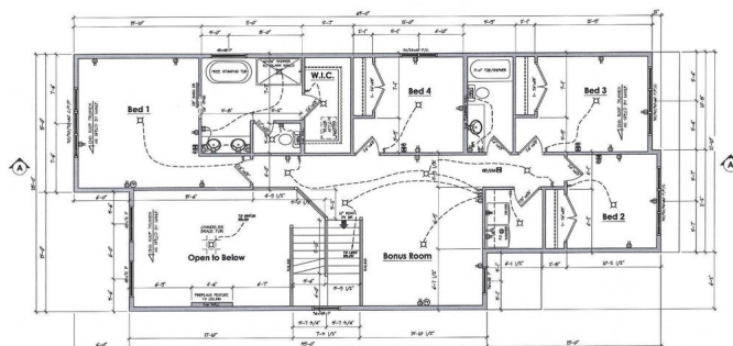
Second Floor Plan 1206 of 1206 8 FT Ceiling
